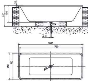
NB25801W NB25801W-A (with overflow function) 1.8m Acrylic Drop-in Bathtub Color: White Material: Acrylic Recommended Products: Copper-texture & Chromium-color bouncing drainer and connecting pipe of bathtub drainer. Size: 1800x750x490mm
