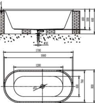
NB25702W NB25702W-A (with overflow function) 1.7m Acrylic Drop-in Bathtub Color: White Material: Acrylic Recommended Products: Copper-texture & Chromium-color bouncing drainer and connecting pipe of bathtub drainer. Size: 1700x800x500mm
