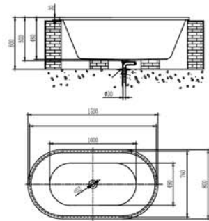
NB25503W NB25503W-A (with overflow function) 1.5m Acrylic Drop-in Bathtub Color: White Material: Acrylic Recommended Products: Copper-texture & Chromium-color bouncing drainer and connecting pipe of bathtub drainer. Size: 1500x800x500mm
