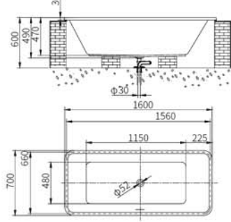
NB25603W (with overflow function) 1.6m Drop-in Bathtub Color: White Material: Acrylic Recommended Products: Copper-texture & Chromium-color bouncing drainer and connecting pipe of bathtub drainer. Size: 1600x700x490mm
