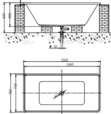
NB25501W NB25501W-A (with overflow function) 1.5m Acrylic Drop-in Bathtub Color: White Material: Acrylic Recommended Products: Copper-texture & Chromium-color bouncing drainer and connecting pipe of bathtub drainer. Size: 1500x750x490mm
