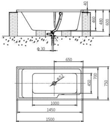
NB25502W (with overflow function) 1.5m Acrylic Drop-in Bathtub Color: White Material: Acrylic Recommended Products: Chromium-color bathtub hand-wheel drainer and connecting pipe of bathtub drainer. Size: 1500x750x480mm
