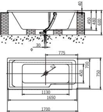
NB25706W (with overflow function) 1.7m Acrylic Drop-in Bathtub Color: White Material: Acrylic Recommended Products: Chromium-color bathtub hand-wheel drainer and connecting pipe of bathtub drainer. Size: 1700x750x480mm
