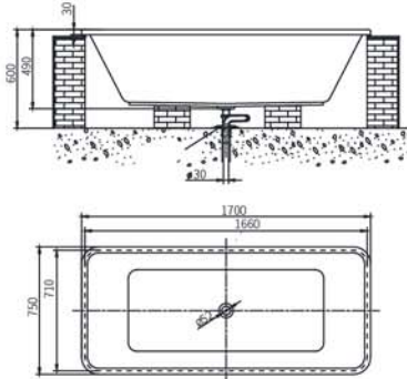
NB25703W NB25703W-A (with overflow function) 1.7m Acrylic Drop-in Bathtub Color: White Material: Acrylic Recommended Products: Copper-texture & Chromium-color bouncing drainer and connecting pipe of bathtub drainer. Size: 1700x750x490mm
