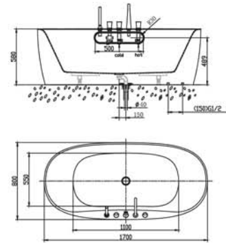
NB25714M-1 NB25714W-1A 1.7m Free Standing Bathtub Color : Matt White/White Material : Acrylic Included : With overflow function,Contains Black/Chrome copper bouncing water dispensers, Chrome overflow grooves and connecting pipe of bathtub drainer. NF52370C/K-5, 5-pc Windespread Bath Faucet. Size: 1700x800x580mm
