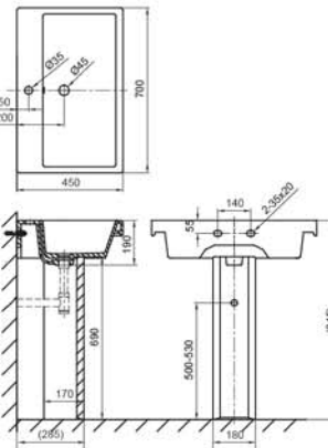
70cm Basin(1-Hole) +Pedestal Size: NC2214W-1: 700x450x190mm NCE01W : 180X170X690mm Material:Vitreous china
