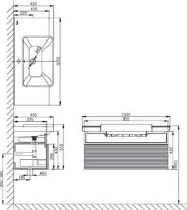
1. 100cm Vanity Top (Vitreous China) 2. 100cm Wall-hung Vanity Color: Canadian grey Size: 1000x450x510mm Material: Plywood Structure: Double Drawers Key Parts: DTC Soft Closing Tracks
