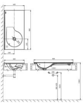
90cm Drop-in Basin (1-Hole) Size: 900x465x175mm Material: Vitreous china 90公分柜盆 (单孔) 尺寸: 900x465x175mm 材质: 陶瓷
