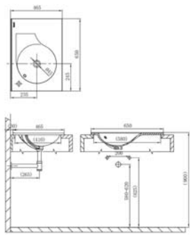
65cm Drop-in Basin (1-Hole) Size: 650x465x175mm Material: Vitreous china 65公分柜盆 (单孔) 尺寸: 650x465x175mm 材质: 陶瓷
