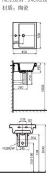
50cm Basin(1-Hole) + Semi Pedestal Size: NC2213W-1: 500x450x190mm NCE02W: 245X280X250mm Material: Vitreous china 50公分盆(单孔)+半底座 尺寸: NC2213W-1: 500x450x190mm NCE02W: 245X280X250mm 材质: 陶瓷
