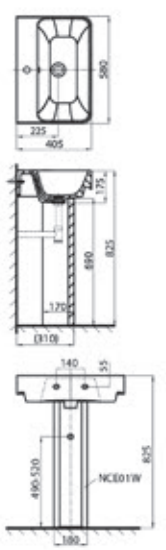
58cm Basin(1-Hole) + Pedestal Size: NC2259W-1: 580x405x175mm NCE01W: 180X170X690mm Material: Vitreous china 58公分盆(单孔)+底座 尺寸: NC2259W-1: 580x405x175mm NCE01W: 180X170X690mm 材质: 陶瓷
