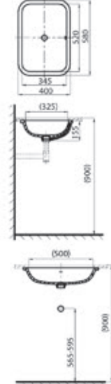
58cm Rectangle Under-mount Basin Size: 580x400x155mm Material: Vitreous china 58公分方形台下盆 尺寸: 580x400x155mm 材质: 陶瓷
