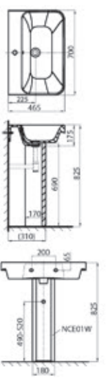
70cm Basin(1-Hole) + Pedestal Size: NC2260W-1: 700x465x175mm NCE01W: 180X170X690mm Material: Vitreous china 70公分盆(单孔)+底座 尺寸: NC2260W-1: 700x465x175mm NCE01W: 180X170X690mm 材质: 陶瓷
