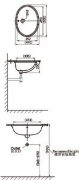
55cm Under-mount Basin Size: 550x410x200mm Material: Vitreous china 55公分台下盆 尺寸: 550x410x200mm 材质: 陶瓷
